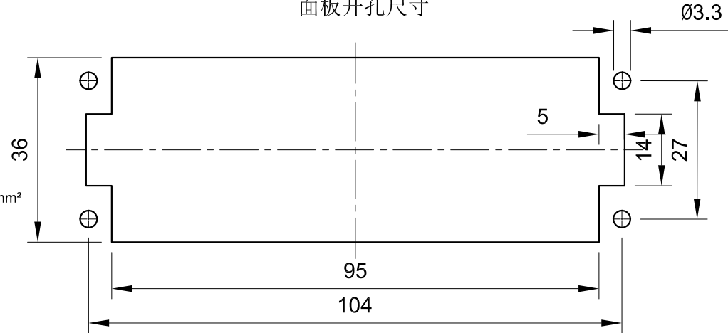
Panel cut out 面板开孔尺寸
